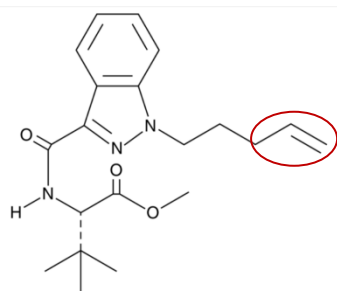
MDMB-4en-PINACA
